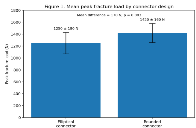
Figure 1. Mean peak fracture load of elliptical and rounded connector designs
